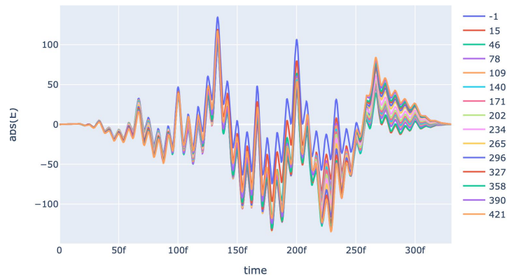
Absolute value of the laser field envelope
